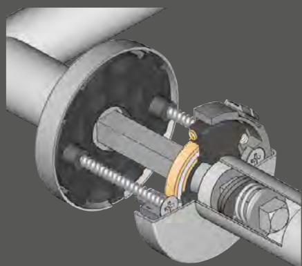
BB Schlüsselrosette
